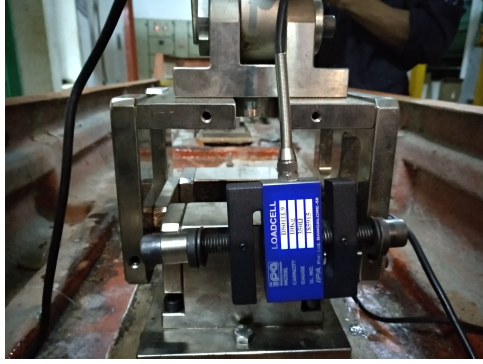
FIGURE 12. loadcell mounting arrangement: actual setup
