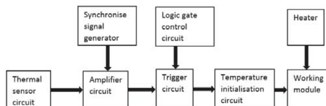
Fig. 1 System structure
