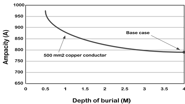
Fig. 10 Ampacity rating versus depth of burial
