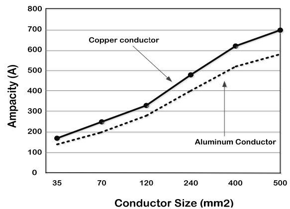
Fig. 12 Ampacity rating versus conductor size for both (aluminum and copper conductors)
