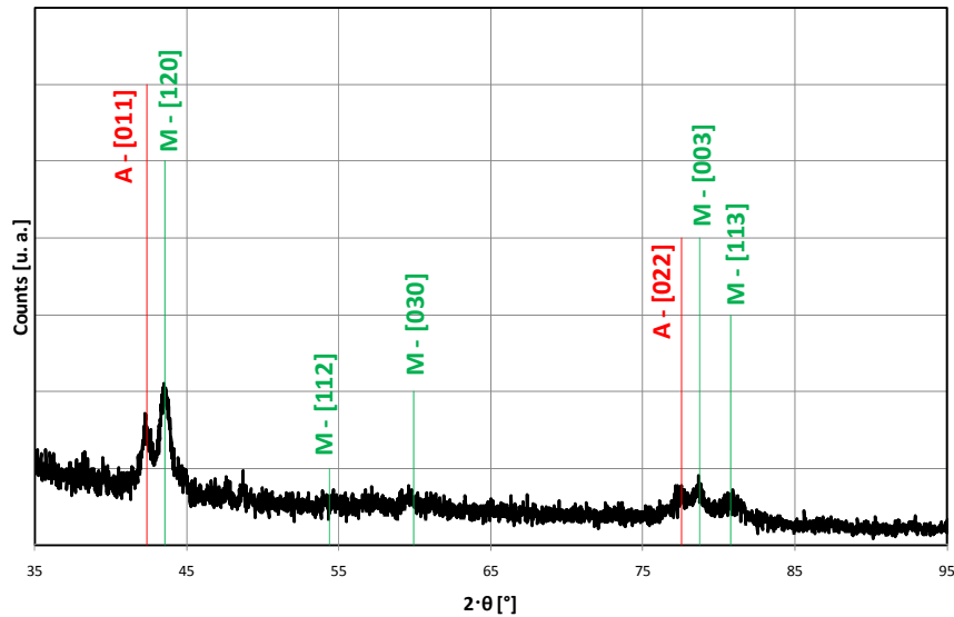
Figure 11: X-Ray spectra of obtained from unloading from \epsilon_g=10\% to \epsilon_g=5\% .
