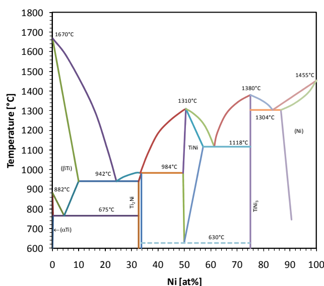
Figure 1: NiTi alloy phase diagram.
