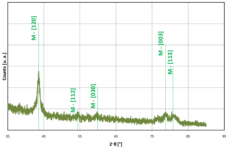
Figure 10: X-Ray spectra obtained from monotonic loading up to \epsilon_g=10\% .
