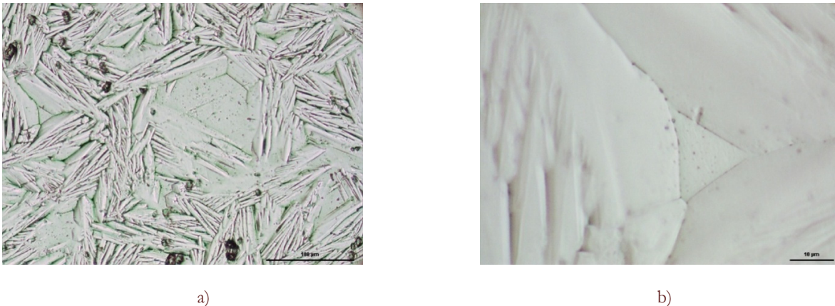
Figure 2: Initial austenitic microstructure of the investigated NiTi alloy: a) at low magnification showing the presence of inclusions, b) high magnification with presence of subgrains.
