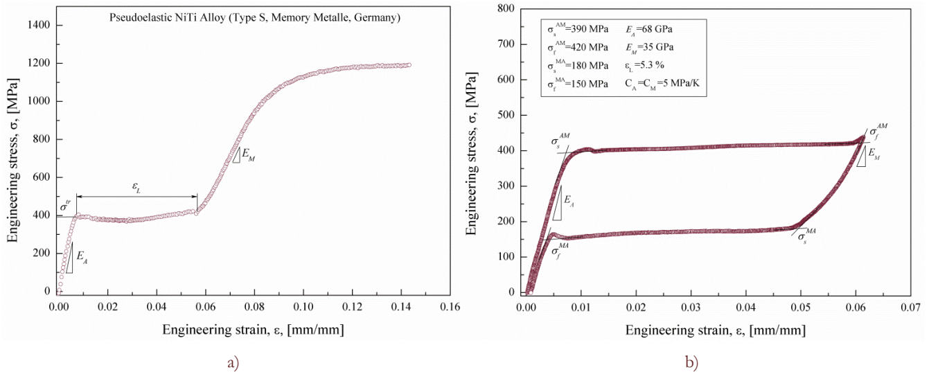
Figure 3: Isothermal stress-strain curve of the investigated alloy carried out at room temperature ( T=298 k): a) monotonic loading to fracture and b) loading-unloading cycle.
