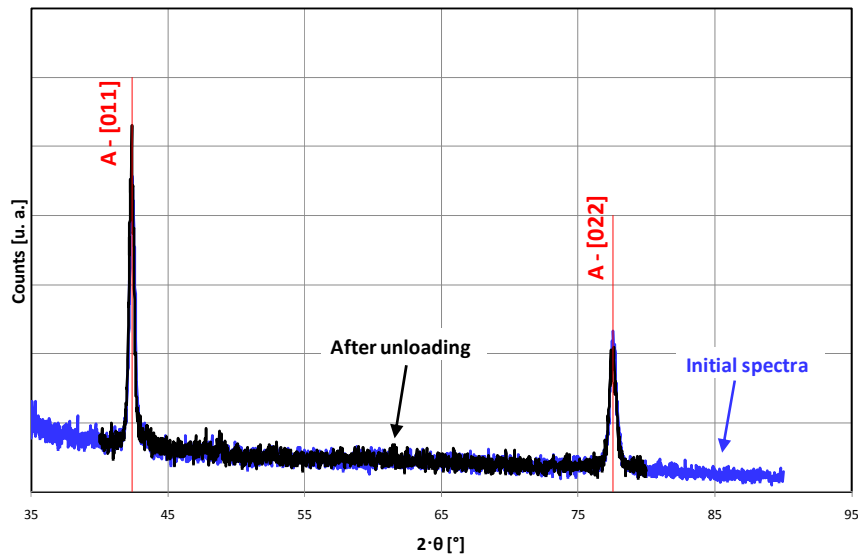
Figure 12: Comparison of the X-Ray spectra between initial condition and final stress free condition after unloading.
