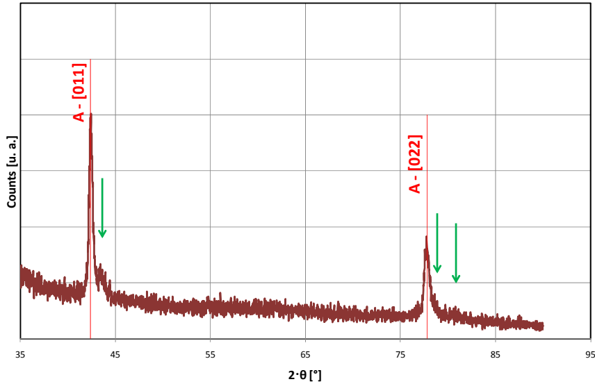
Figure 9: X-Ray spectra obtained from monotonic loading up to \epsilon_g=5\% .
