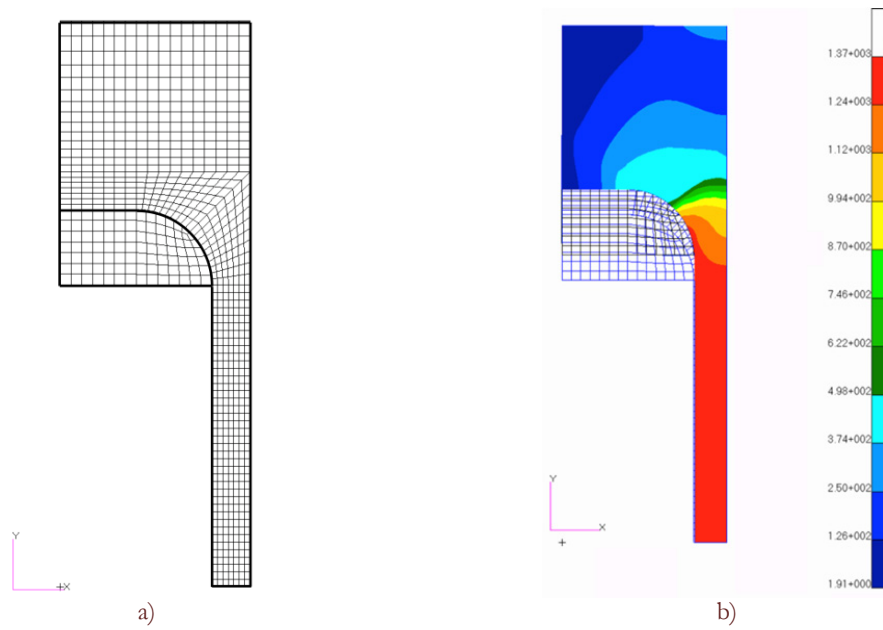
Figure 5: FE analysis of the testing condition: a) FE model and b) equivalent stress fringes at the maximum elongation.
