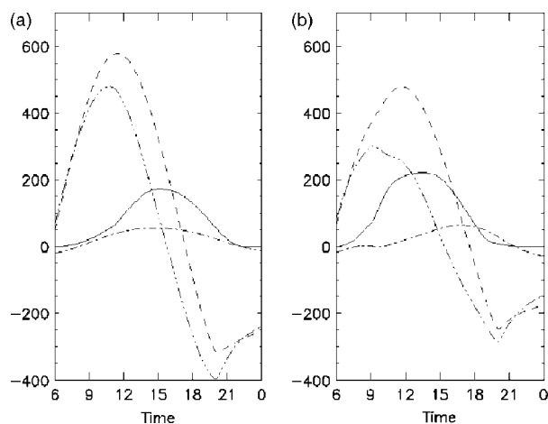
Figure 12. Idealized MetUM outputs of surface energy balance fluxes ( W m^{-2} ) for the new scheme with (a) thick and (b) thin roofs. The line styles are as in Figures 7 and 8. See text for further explanation.
