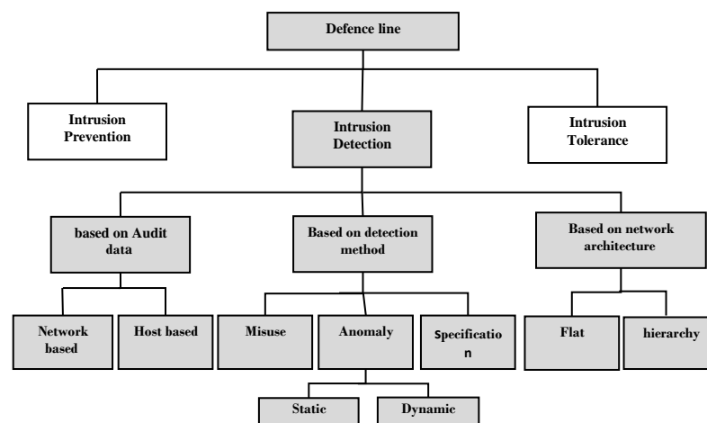
FIGURE 1. Classification of IDS
