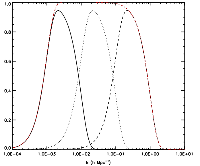
Figure 5. Three filters used to calculate the contribution of the different modes to the correlators, their variance, and the SN ratio. The filters have \{k_l = 10^{-3}, k_L = 10^{-2}\} (solid curve), \{k_l = 10^{-2}, k_L = 10^{-1}\} (dotted curve), and \{k_l = 10^{-1}, k_L = 1\} (dashed curve). Also shown is the sum of the filters (red dash-dotted curve).
