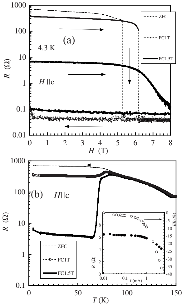
FIG. 3. (a) ab -plane MR data of the z=0.6 crystal after the field cooling runs, FC-1 T and FC-1.5 T, at 0.1 mA ( H\parallel c ). For comparison, the ZFC data are presented. (b) The temperature profile of the resistance monitored in the FC process from 150 down to 4 K. The inset presents the ER and the ER ratio in the FC-1.5 T case at 4.3 K.
