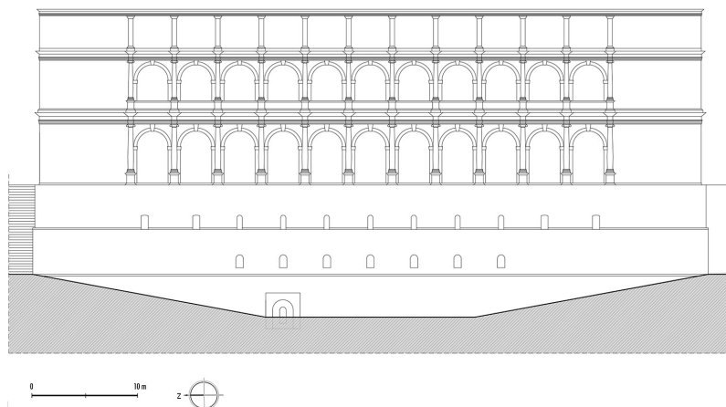
FIG. 14. Reconstruction of the western façade of the forum of Aeminium (by Alarcão et al., 2009).
