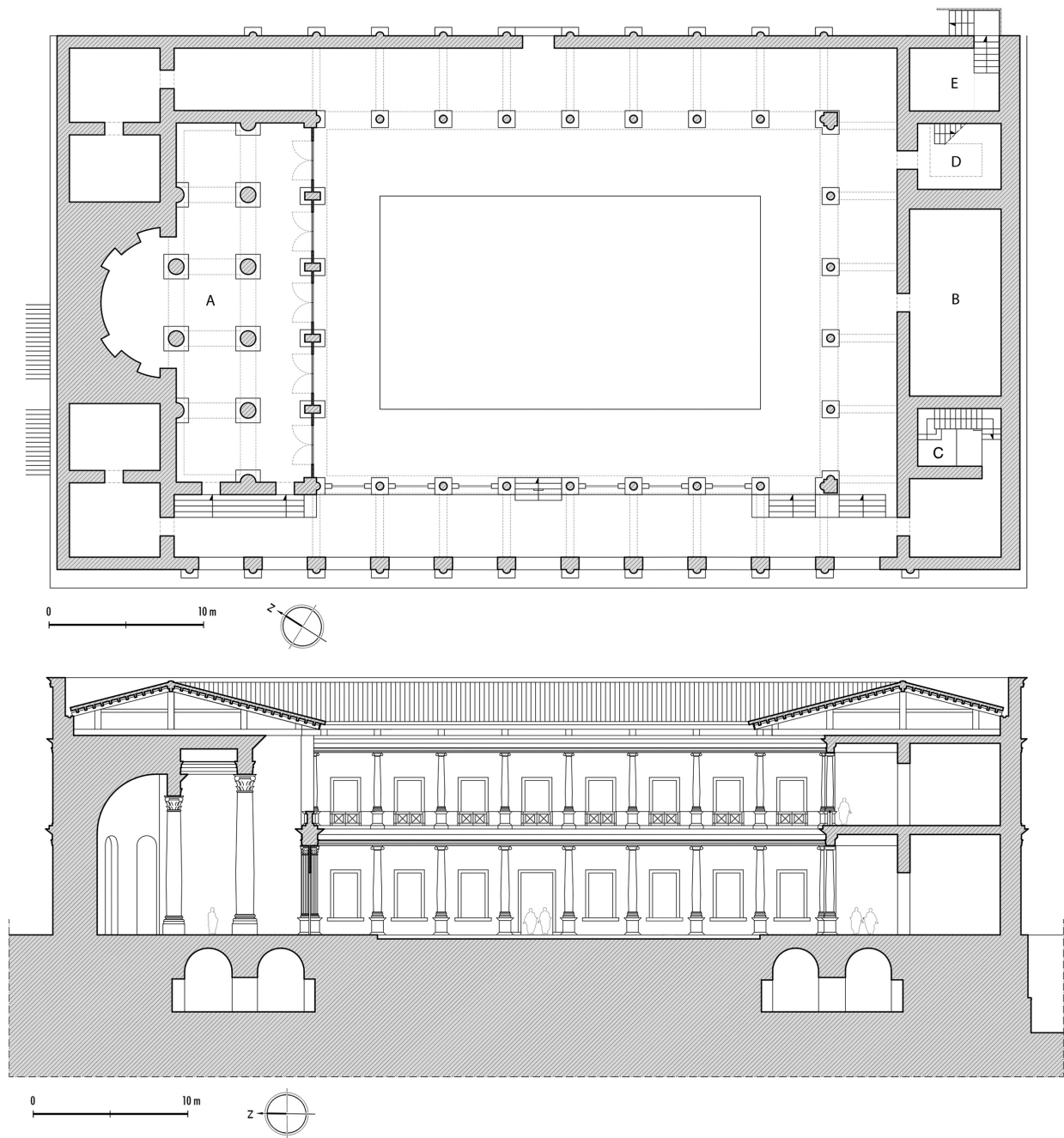
FIG. 18. Plan of the forum of Aeminium on the level of the area publica and reconstruction of the elevation from the median longitudinal axis (by Alarcão et al., 2009).
