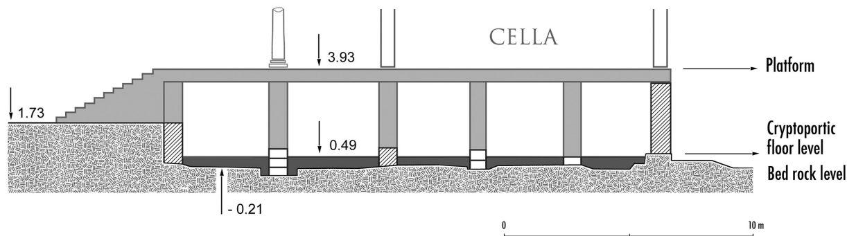
FIG. 3. Cross-section of the Augustan cryptoportico of Conimbriga, with the hypothetical reconstruction of the staircase giving access to the platform and of the level at which it is found.
