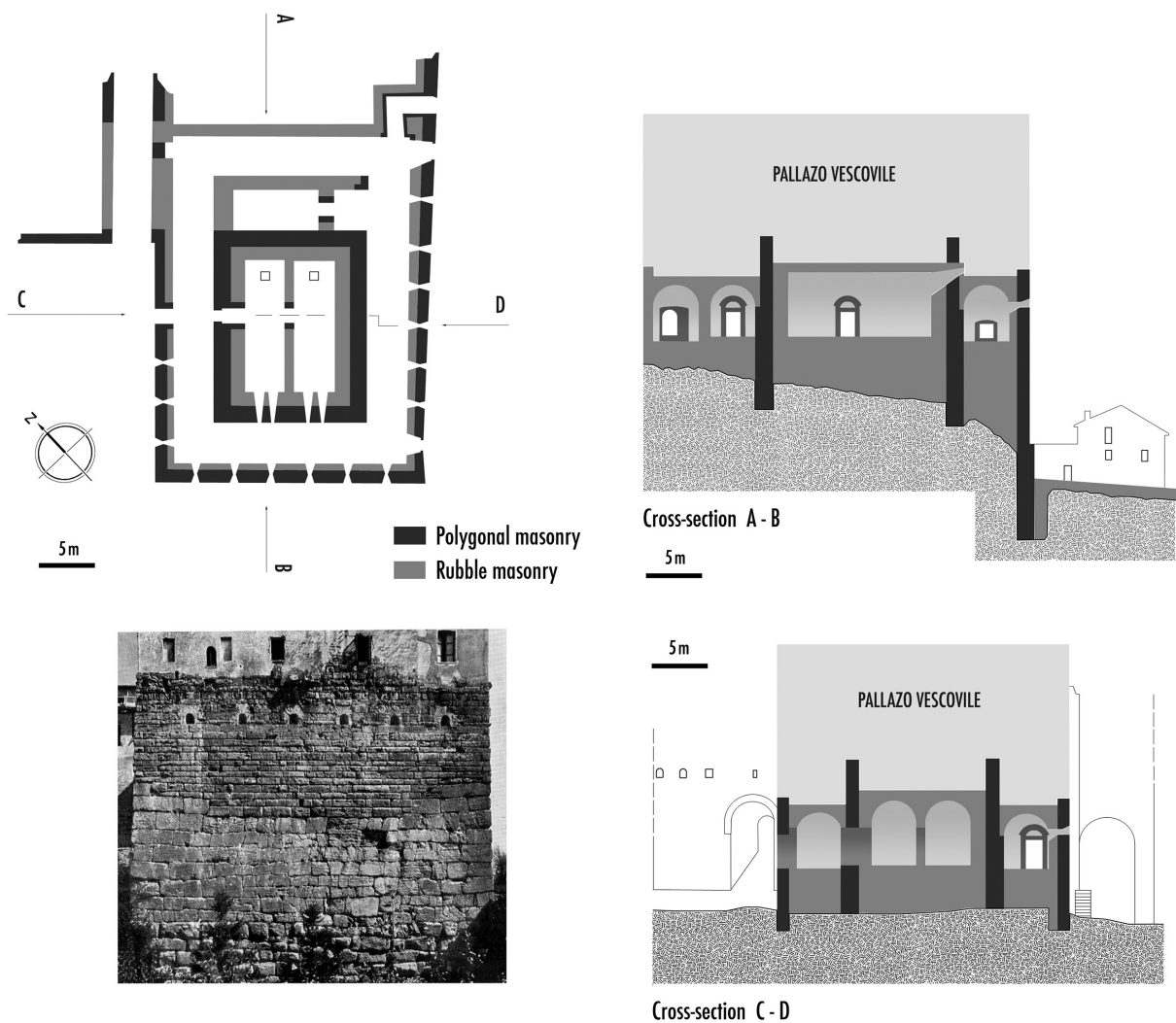
FIG. 15. Cryptoportico of Ferentino (redrawn on Gullini, 1954).
