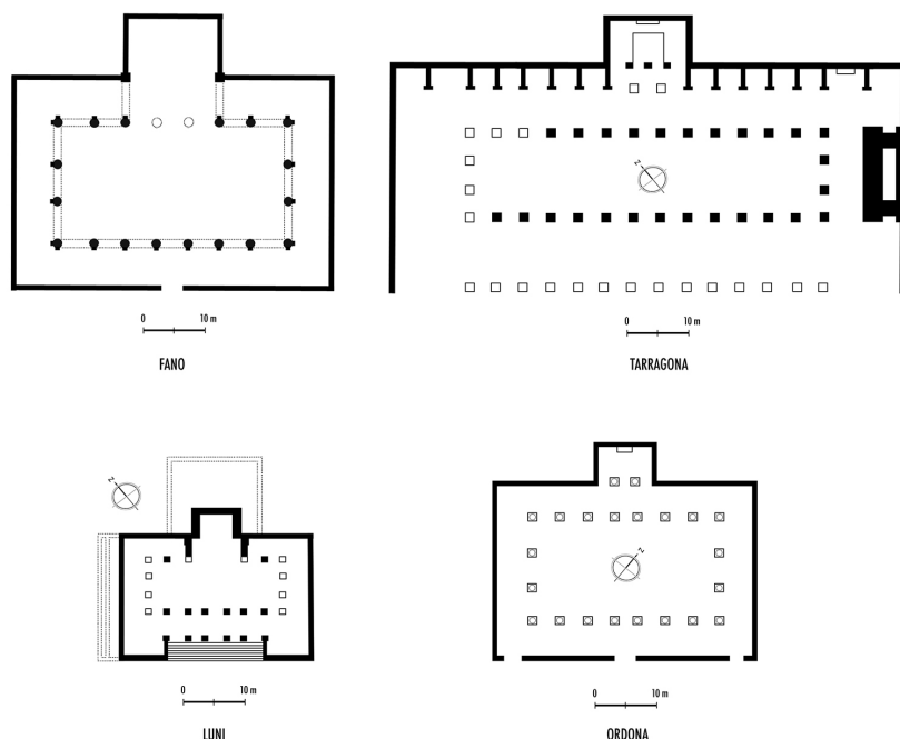
FIG. 6. Basilicas of Fano, Tarraco, Luna and Herdonia, drawn to the same scale (from plans presented by Balty, 1991).
