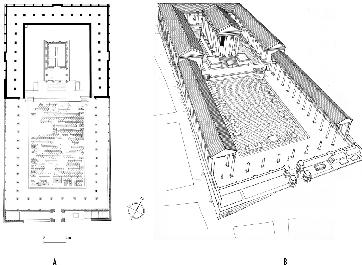
FIG. 10. Plan and reconstruction of the Flavian forum of Conimbriga (by Alarcão and Étienne, 1977).
