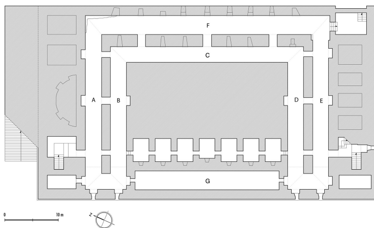
FIG. 12. Plan of the upper floor of the cryptoportico of Aeminium.
