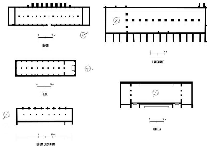
FIG. 8. Basilicas of Noviodunum, Lousona, Veleia, Iulium Carnicum and Thera (by Balty, 1991 and Hauser and Rossi, 1998).
