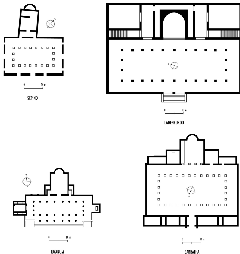
FIG. 7. Basilicas of Saepinum, Lopodunum, Iuvanum and Sabratha (from plans presented by Balty, 1991).
