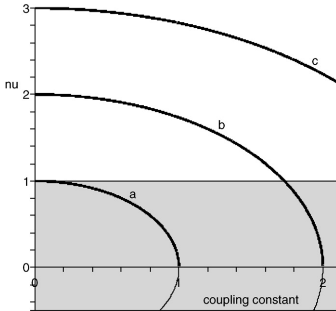
Fig. 2. The solutions of the system of indicial equations, \nu_+ (thick line) and \nu_- (thin line), as a function of the coupling constant for the Dirac case (a for |\kappa| = 1 , b for |\kappa| = 2 and c for |\kappa| = 3 ). The shaded area represents the zone corresponding to radial solutions diverging at the origin.
