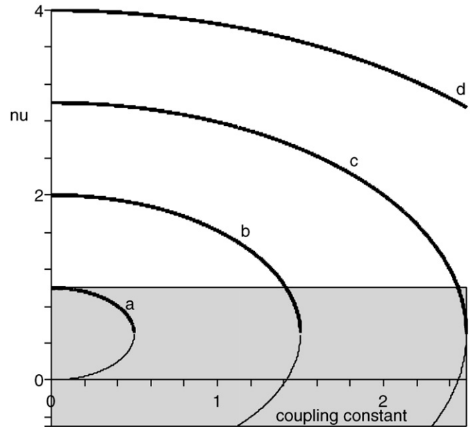
Fig. 1. The roots of the indicial equation, \nu_+ (thick line) and \nu_- (thin line), as a function of the coupling constant for the Klein–Gordon case (a for l = 0 , b for l = 1 , c for l = 2 and d for l = 3 ). The shaded area represents the zone corresponding to radial solutions diverging at the origin.
