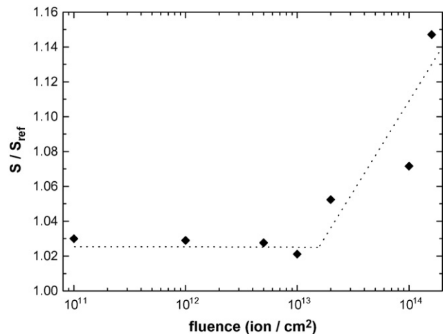
Fig. 2. The S values of irradiated sapphire samples normalized to the defect-free reference sample in the fluence range of 10^{11} – 1.6 \times 10^{14} ion cm -2 . The line is only to guide the eyes.
