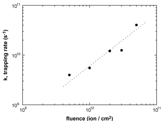
Fig. 3. Overall positron trapping rates in monovacancies as a function of fluence inside the cylindrical volume around the ion track. Fluence range: 5 \times 10^9 – 5 \times 10^{10} ion \text{cm}^{-2} . The line serves only to guide the eyes.
