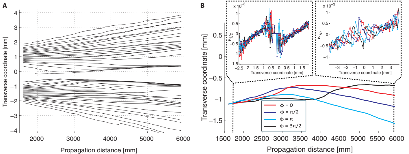
Fig. 3. Observation of nonlocality in Bohmian mechanics. (A) The reconstructed trajectories when photon 2 is found in the state |A\rangle = \frac{1}{\sqrt{2}}(|H\rangle - |V\rangle) . The trajectories are drawn over a range of z = 1.7 m to z = 5.9 m, using 67 different planes. The state of photon 1 after postselection contains no information about the state of photon 2, and thus, interference is observed. (B) A single postselected trajectory beginning at the same initial condition, x = -1.12 mm, for four different postselected polarization states of photon 2, \frac{1}{\sqrt{2}}(|H\rangle - e^{i\Phi}|V\rangle) , where \Phi \in \{0, \pi/2, \pi, 3\pi/2\} . The pairs \{0, \pi\} and \{\pi/2, 3\pi/2\} correspond to measuring the polarization of photon 2 in two different bases. (Inset) The weak velocity values measured at z = 1.8 m and z = 5.9 m. The velocity distributions are initially independent of phase shift applied to photon 2 but depend strongly on it in the far field. The error bars on the individual velocity measurements are consistent with the scatter observed but are not displayed because they detract from rather than enhance its clarity.
