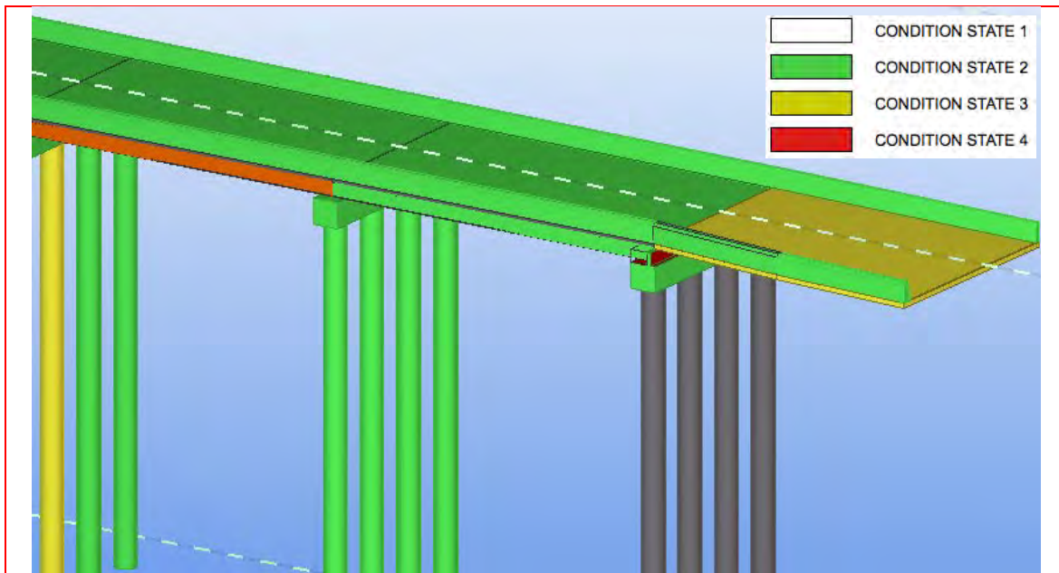
Fig. 4 Revit model with condition information assigned
