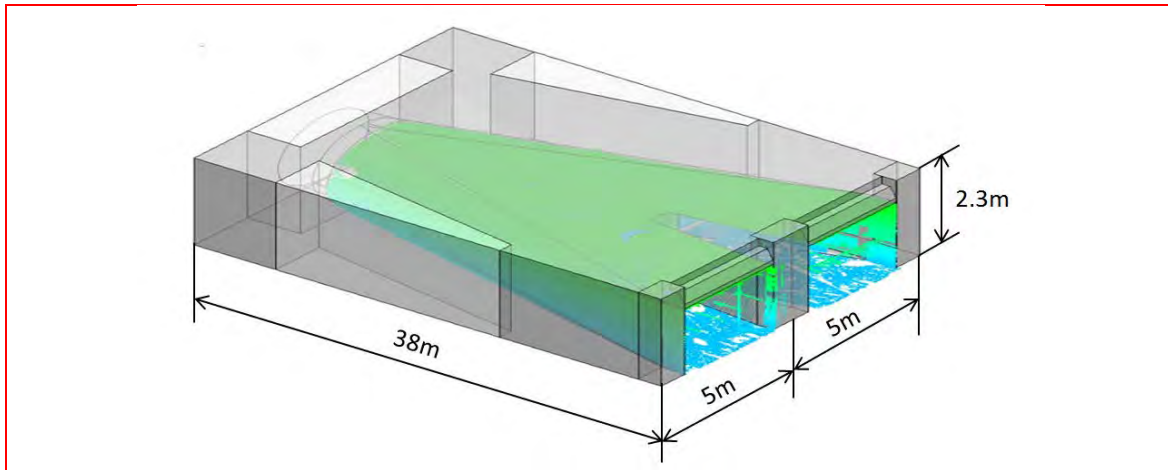
Fig. 6 3-D point cloud model overlay within BIM model
