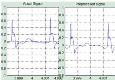
Fig. 6. Denoising
