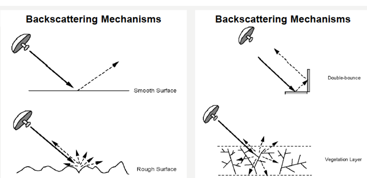
Figure 3. Various types and styles of backscattering mechanisms that contribute to the strength of signal received, as a function of what has been sampled.
