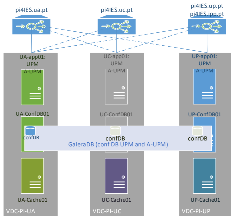
Figure 4 VDC-PI4IES architecture
