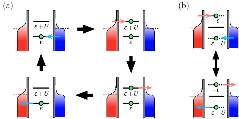
Figure 5. Sketch of the processes leading to Fourier heat transfer in the thermally broadened region around the particle-hole symmetry point, \varepsilon - \mu = -U/2 , for (a) the normal and (b) the inverted quantum dot models. In both cases shown, the energy U flows from the hot lead to the cold one without net charge transfer from the left to the right lead.
