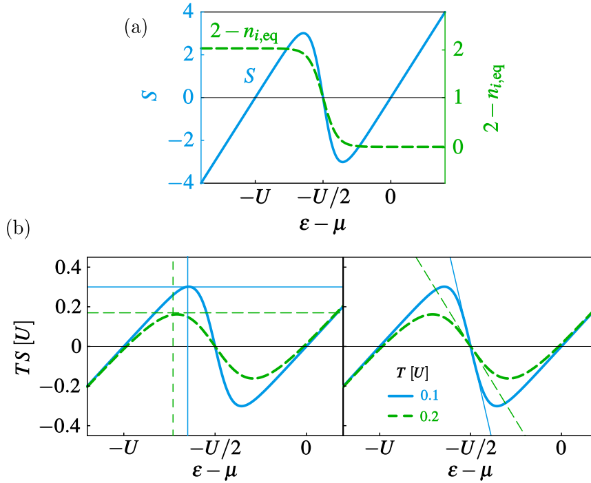
Figure 3. (a) Linear Seebeck thermopower S , Eq. (31), (solid-blue line), and 2 - n_{i,\text{eq}} (dashed-green line) as a function of the level position of the dot \varepsilon - \mu , for U = 10T . Here, n_{i,\text{eq}} is the occupation number of the inverted stationary state at equilibrium. In the units chosen here ( e = k_B = 1 ), the Seebeck coefficient is dimensionless. (b) Comparison with the approximate position and height of the local maxima of S , given by Eq. (34), (left panel), and of the slopes at the particle-hole symmetry point, given by Eq. (35), (right panel). For all panels, the couplings are chosen \Gamma_L = \Gamma_R \ll T .
