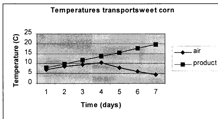
Figure 1: influence of transport time on the air and product temperature during transport in a Reefer container from Israel to The Netherlands.
