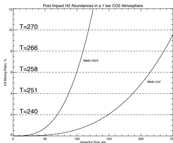
Figure 1. \text{H}_2 mixing ratios (%) vs impactor size (km). Dotted horizontal lines labeled T=270 , 266, etc. correspond to the global mean temperatures from [2] for a 1 bar \text{CO}_2 atmosphere with the indicated hydrogen mixing ratio. Melt is the volume of melt material, and V is the volume of the impactor.
