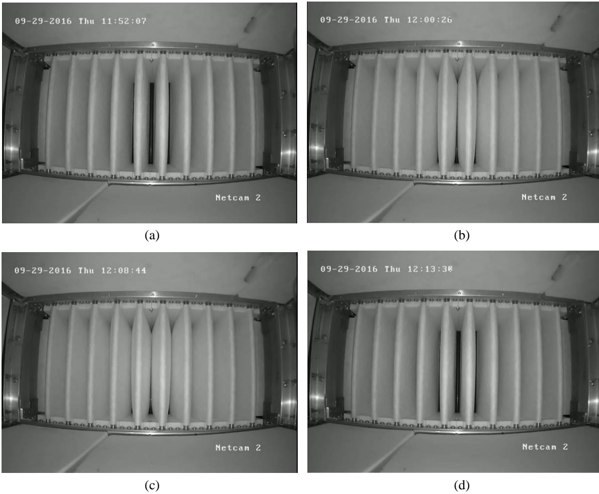
Figure 6. Video still images of the SMF in the REMS module. a) 2 m 3 /min, b) 4.2 m 3 /min, c) 6.2 m 3 /min, and d) no flow.
