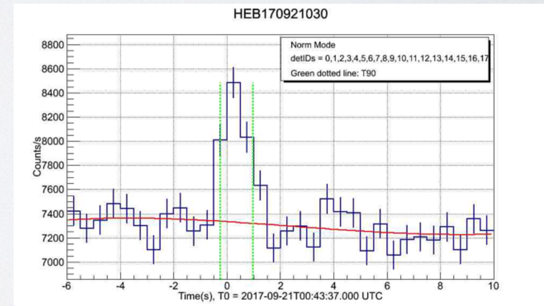
Insight-HXMT lightcurve
