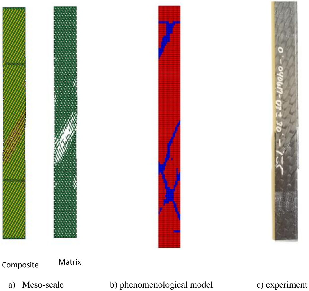
Figure 12: Crack Paths in a [30/-30/-30/30] Laminate Coupon
