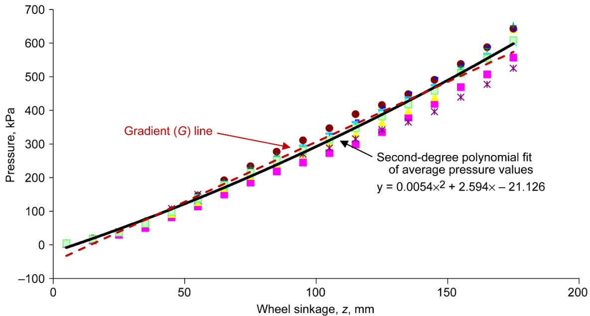
Figure 7.—Typical cone penetrometer results for the T2 terrain condition. Eight data sets are shown together with a second-degree polynomial fit of the average penetration-resistance-versus-depth data points. Cone index gradient, G = 3.57 \text{ kPa/mm} ; standard deviation = 0.286 \text{ kPa/mm} ; linearity coefficient = 0.0054 \text{ kPa/mm}^2 .
