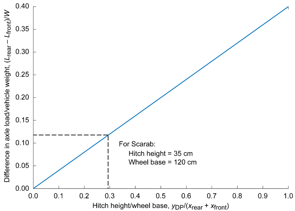
Figure 22.—Estimated effect of hitch height on load transfer at drawbar pull (DP) force coefficient F_{DP}/W = 0.2 . (The center of gravity is centered between front and rear axes.)
