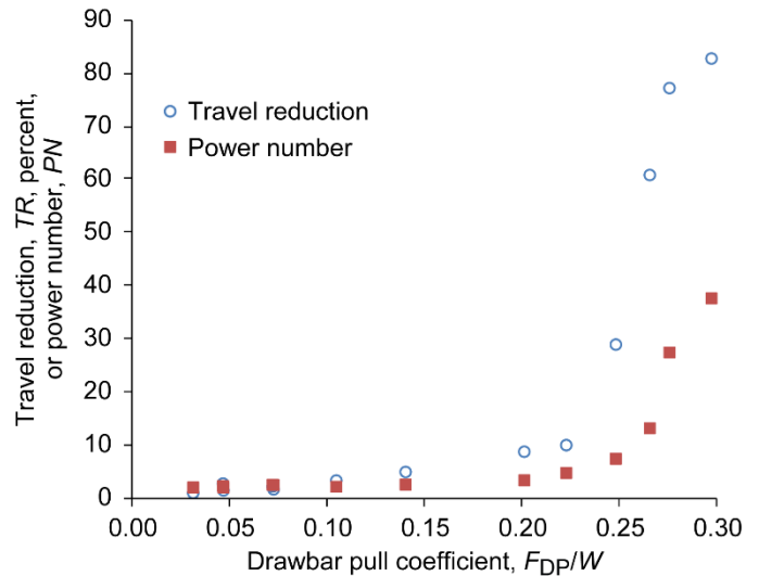
Figure 5.—Results of drawbar pull (DP) test, displaying travel reduction and power number as functions of the DP coefficient.
