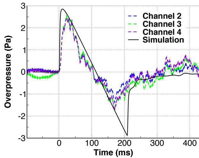
Figure 12. Observed and computed ground pressure signatures for the Stardust capsule. Each “Channel” corresponds to a sensing microphone.
