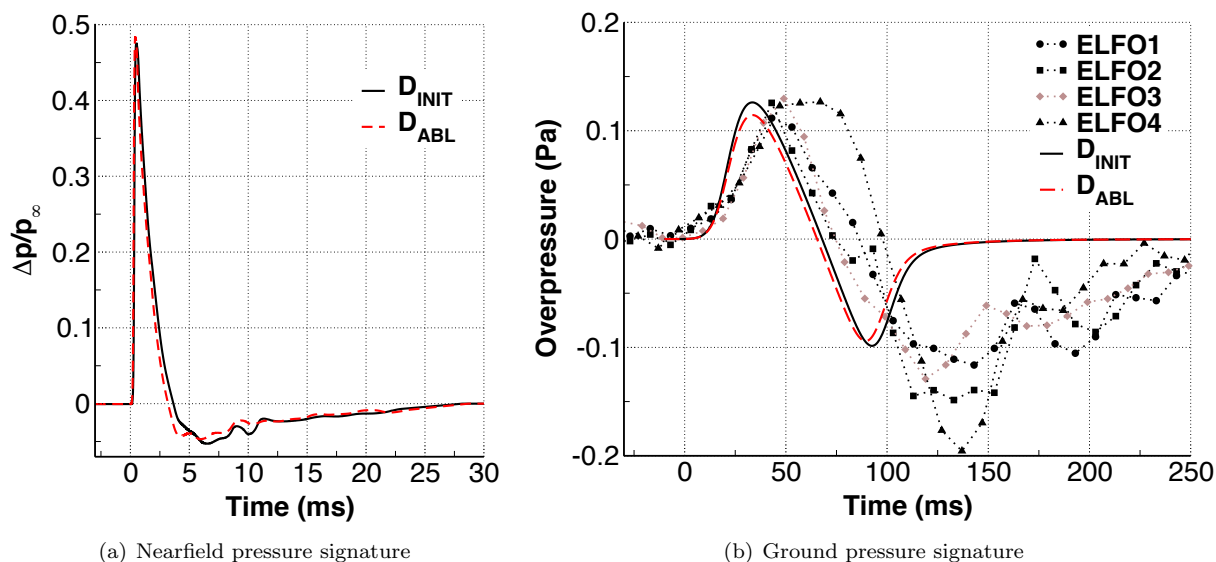
Figure 15. Nearfield and ground pressure signatures for the first arrival from Meteor 20090428. Results for the initial and ablated shapes are shown, labeled “ D_{INIT} ” and “ D_{ABL} ”, as well as ELFO observations from 4 sensors. Nearfield signature extracted at distance of 40D ( M_\infty = 67.5 and H = 58.7 km).
