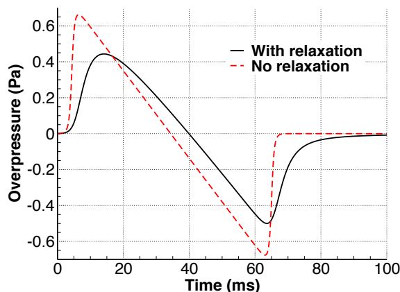
Figure 7. Ground signatures with and without molecular relaxation losses.
