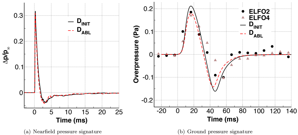
Figure 14. Nearfield and ground pressure signatures for Meteor 20081028. Results for the initial and ablated shapes are shown, labeled “ D_{INIT} ” and “ D_{ABL} ”, as well as observations from two ELFO sensors, labeled “ELFO2” and “ELFO4”. Nearfield signature extracted at distance of 40D ( M_\infty = 45.6 and H = 53.7 km).
