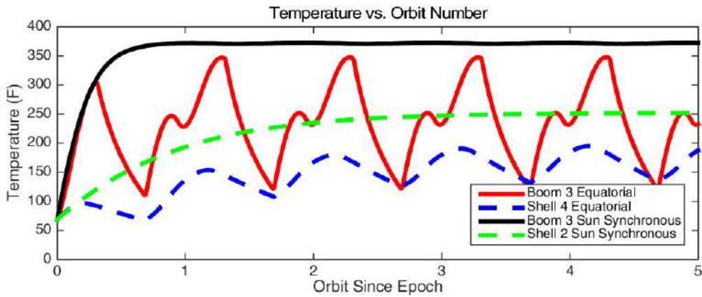
Figure 19: On-Orbit Temperatures Estimated via Numerical Simulations
