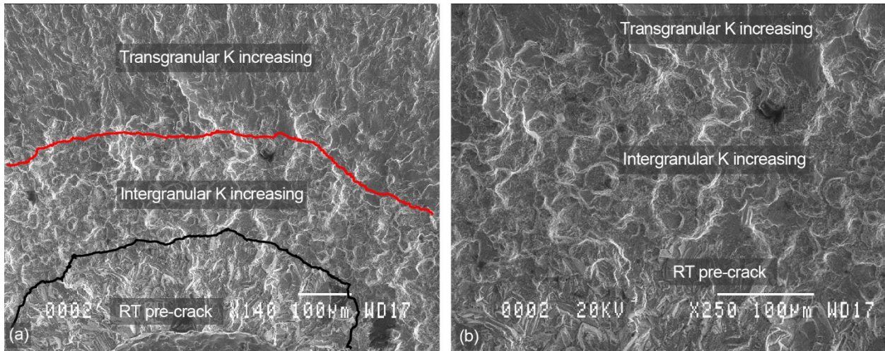
Figure 13.—LSHR short pre-crack, K increasing (K incr) test at 704 °C and 0.667 Hz at (a) low and (b) higher magnifications. Initial intergranular failure mode followed by sudden transition to mostly transgranular failure.
