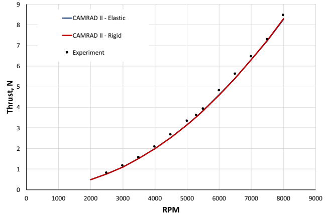
Figure 7. Predicted thrust for DJI Phantom 3 rotor.
