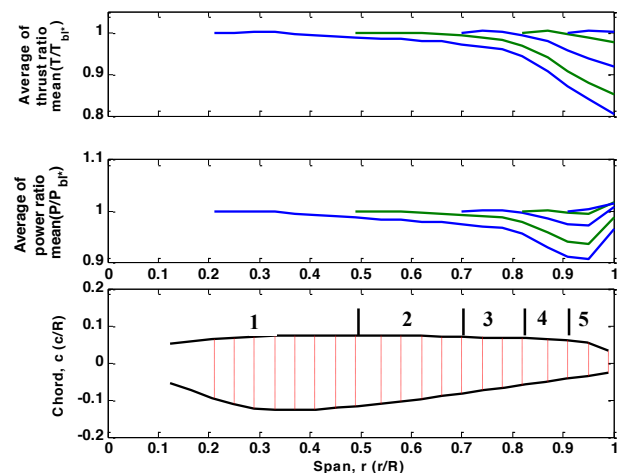
Figure 19. Change in thrust and power ratio due to changes in airfoil distribution, free wake, \theta_0 = -1 deg, \Delta TR_{lim} = 0.01 .
