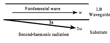
Fig. 1. Schematic diagram of the Čerenkov-type configuration.
