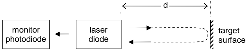
Figure 1. Typical schematic configuration for measurement of deflection using laser diode self-mixing. After Guiliani et al [4] .
