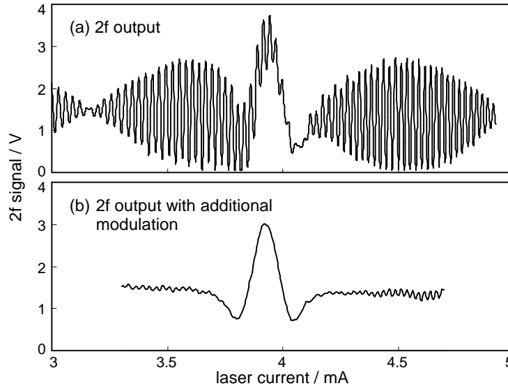
Figure 18. 2f WMS signals acquired by the microLGD TM for a methane concentration of 100ppm. (a) Interference fringes superimposed on the absorption line for straightforward WMS at f=20 kHz. (b) Suppression of fringes using an additional low amplitude modulation.
