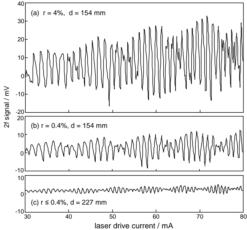
Figure 10. Self-mixing induced interference fringes observed in the laser diode forward emission for feedback from (a) an uncoated 6^\circ wedged window at a distance of 154mm, (b) an AR coated 6^\circ wedged window at a distance of 154 mm, and (c) the latter at a distance of 227 mm.
