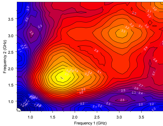
Figure 3. Combined 1g SAR with two vertical dipoles
