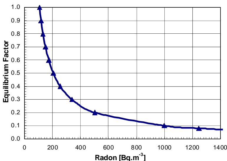
Fig. 4. Iso-Risk Plot (Excess Risk = 0.008) for Males in 200 Bq.m -3 , EF = 0.5 Environment.
