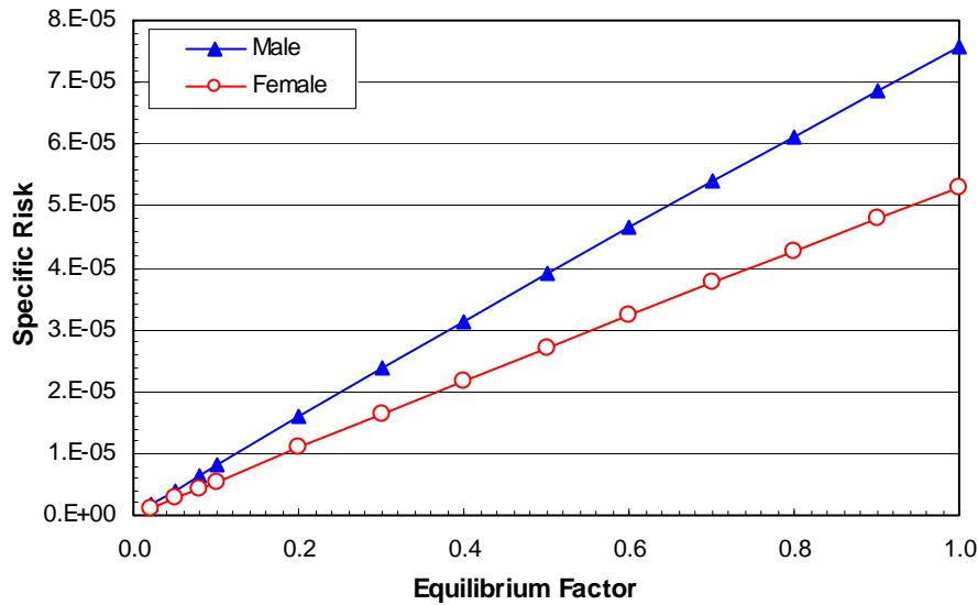
Fig. 1. Variation of excess risk per unit \text{Bq.m}^{-3} radon concentration, linear in radon over the range 0 – 1000 \text{ Bq.m}^{-3} , with Equilibrium Factor for 40-year-old non-smoking Males and Females
