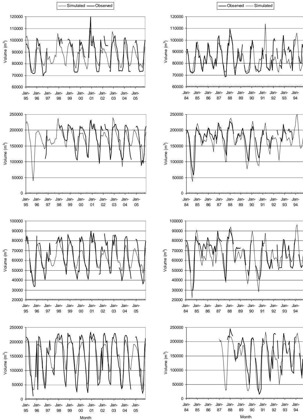
Figure 7 Simulated and observed lake volumes in the (from top) Upper Eastern Arm; Lower Eastern Arm; Central Arm; Central Lake-Western Arm during the (left) calibration and (right) validation periods.
