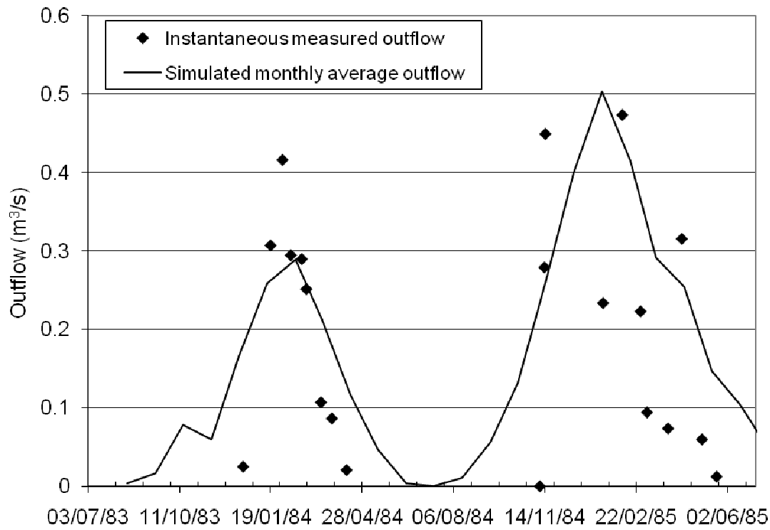
Figure 8 Modelled monthly average and instantaneous measured lake outflows to the sea during the validation period
