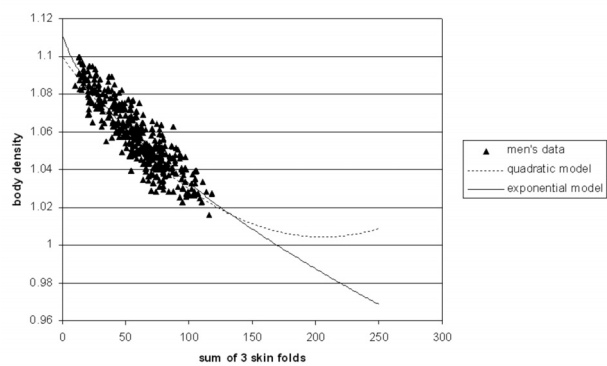
Figure 3. The quadratic model and proposed alternative exponential power-function model for men.
