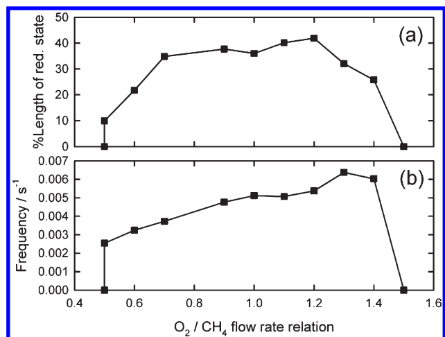
Figure 7. (a) Duration of the reduced state in one oscillation cycle, that is, the average percentage in time of an oscillation period where the catalyst is in the reduced state as a function of the inlet gas composition. (b) Frequency of the oscillations as a function of the O 2 /CH 4 ratio. The FSP catalyst was used with a fixed temperature of 418 °C and measured at the relative position x/L = 0.67 .
