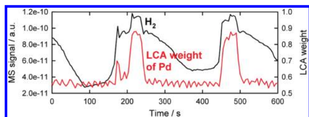
Figure 5. Inner oscillation (superimposed on the actual oscillation of CPO) in hydrogen production and oxidation state of the Pd catalyst at the beginning of the catalyst bed ( x/L = 0 ). Conditions for the FSP catalyst in this case were 418 °C and 27 mL/min of 6% CH 4 /3% O 2 /He.
