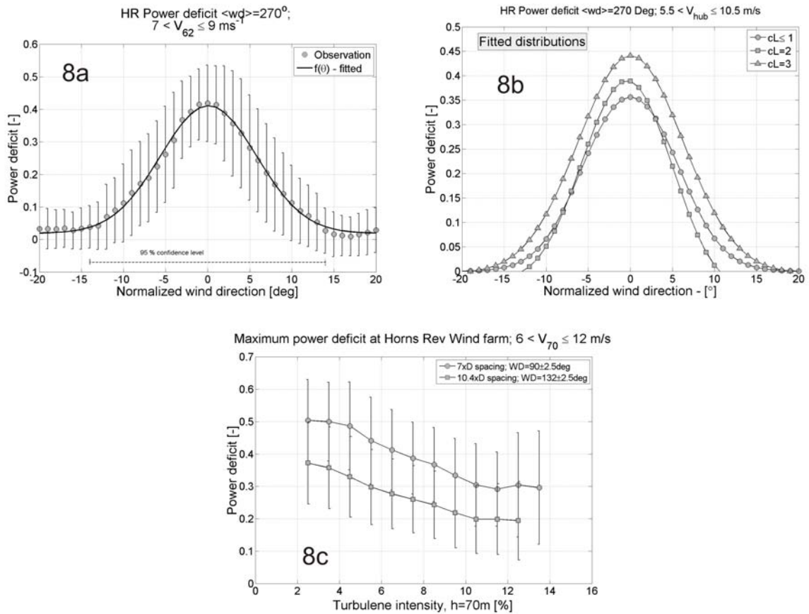
Figure 8: Power deficit at Horns Rev. Figure 8a shows the power deficit distribution as function of normalized wind direction for Horns Rev wind turbine wt17 compared to wt07 (spacing 7D). Turbine locations are shown in Figure 1. Wind speeds were selected with reference to M2 at 62 m for directions 270^\circ in Figure 8a. One standard deviation representing each 5^\circ sector has been included as error bars. Figure 8b shows fitted power deficit distributions for wt17 relative to wt07 - grouped on stability classes; cL=3, 2 & \leq 1 . Figure 8c shows the maximum power deficit for 7D and 10.4D spacing as function of turbulence intensity averaged for a 5^\circ inflow sector. The wind speed interval 6 - 12 \text{ ms}^{-1} and turbulence intensity is measured at M6, 70m and the standard deviation has been included as error bars.
