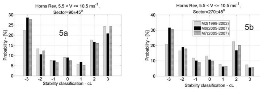
Figure 5: Figure 5a illustrates the free flow stability classification from an eastern direction and Figure 5b illustrates the wake flow classification for a western flow sector. The stability classification at Horns Rev is based on measurements from mast M2, M6 & M7. M2 measurements were recorded during 15.05.1999-14.05.2002 and M6 + M7 measurements represent 3 years (01.01.2005-31.12.2007) with an operating wind farm. Definitions of the stability classes are shown in Table 1.
