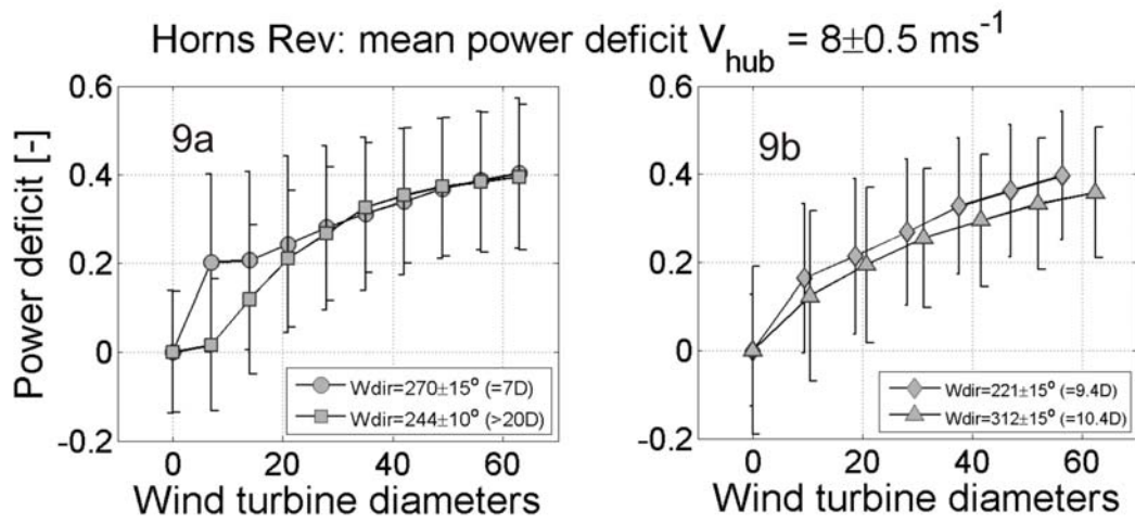
Figure 9: 9a and 9b shows the mean power deficits along rows of wind turbines for different spacing: 7D, 9.4D, 10.4D and >20D, where the curve represents a 30° flow sector except for 244°, which represents a 20° flow sector. The wind speeds range is 8 \pm 0.5 \text{ ms}^{-1} . One standard deviation has been included as error bars.
