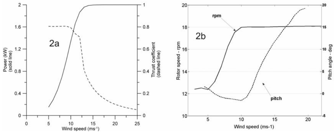
Figure 2: 2a shows the power (P) curve and thrust ( C_T ) coefficient curve for the VESTAS V80 turbine. 2b shows the averaged rotor speed and the average pitch angle both as function of wind speed at hub height.
