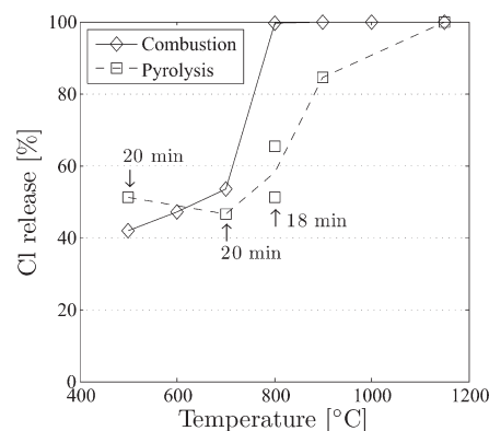
Figure 7. Relative Cl release during pyrolysis and combustion in the temperature range 500–1150 °C. The devolatilization time is 15 min unless otherwise stated.
