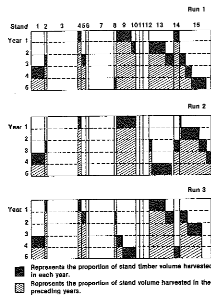
Fig. 1. Optimal harvest schedules for each of the three runs. The area of each stand is drawn to scale to represent the proportion of total forest volume in the stand.
