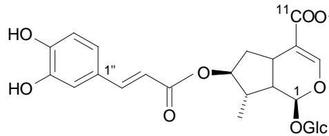
4 lavaudioside C
