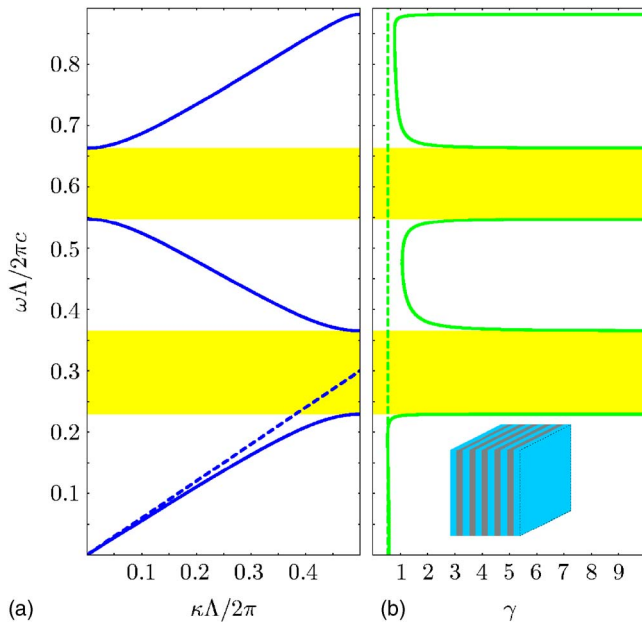
FIG. 2. (Color online) (a) Photonic band structure for normal incidence of either TE or TM polarized light on a Bragg stack of period \Lambda = a_1 + a_2 with n_1 = 1.33 , n_2 = 3 , a_1 = 0.8\Lambda , and a_2 = 0.2\Lambda . Photonic band gaps are indicated by yellow shading and the dashed line indicates the long-wavelength asymptotic limit where \omega \approx c\kappa\Lambda/(a_1n_1 + a_2n_2) . (b) Corresponding enhancement factor which peaks and exceeds unity close to the photonic band-gap edges. The dashed line indicates the long-wavelength asymptotic limit where f = a_1n_1^2/(a_1n_1^2 + a_2n_2^2) .
