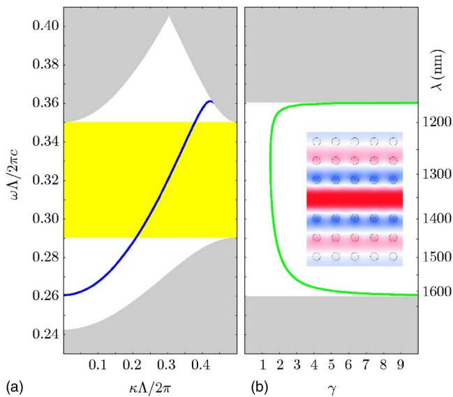
FIG. 4. (Color online) (a) Photonic band structure for propagation of TM polarized light along the \Gamma X direction in a line-defect waveguide in a square lattice of period \Lambda with dielectric rods of diameter d=0.4\Lambda and \epsilon=10.5 . The complete photonic band gap of the photonic crystal is indicated by yellow shading while grey shading indicates the finite density of states in the photonic crystal due to the projected bands in the Brillouin zone. (b) Corresponding enhancement factor which exceeds unity over the entire bandwidth. The right y axis shows the results in terms of the free-space wavelength when results are scaled to a structure with \Lambda=420 nm. The inset shows the electrical field of the waveguide mode at the \Gamma point \kappa=0 .
