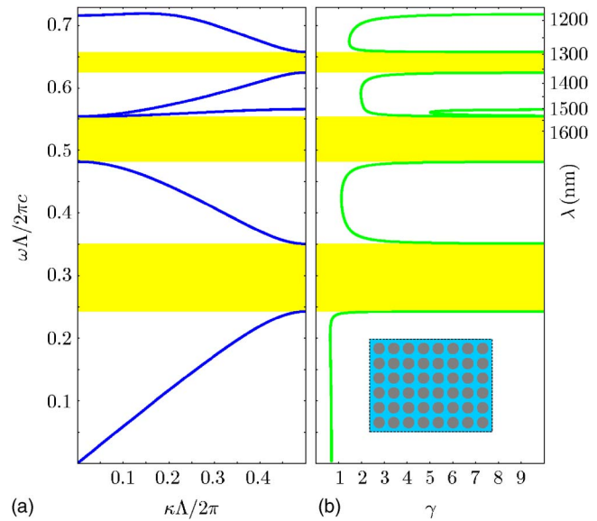
FIG. 3. (Color online) (a) Photonic band structure for propagation of TM polarized light along the \Gamma X direction in a square lattice of period \Lambda with dielectric rods of diameter d = 0.4\Lambda and \epsilon = 10.5 . Photonic band gaps are indicated by yellow shading. (b) Corresponding enhancement factor which exceeds unity for the flat bands in general and the third band in particular. The right y axis shows the results in terms of the free-space wavelength when results are scaled to a structure with \Lambda = 850 nm.
