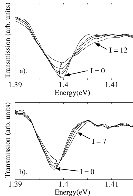
FIG. 3. Experimental transmission of MQW near elh1 exciton with (a) \hbar\omega_{\text{THz}} = 2.5 meV at I_{\text{THz}} = 0, 1, 2, 4, 12 (arbitrary units). (b) \hbar\omega_{\text{THz}} = 14 meV at I_{\text{THz}} = 0, 1, 2, 4, 7 (arbitrary units). Arrows connect calculated centers of experimental peaks and point in the direction of increasing I_{\text{THz}} .
