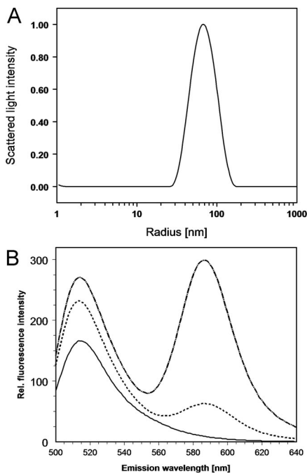
Figure 5. Micelle formation by conjugated primary bile salts (CPBS) and endotoxin binding by these micelles. A , particle size distribution of a 0.05 mM solution of a CPBS mixture. The average radius based on the thermodynamic motility of the micelles was 62.4 \pm 4.3 nm ( n = 8 ). B , fluorescence emission spectra of fluorescein-isothiocyanate (FITC)-labeled endotoxin from Escherichia coli (0.2 mg/mL with 3 \mu g FITC/mg endotoxin; solid line ; emission maximum at 515 nm) in the presence of 0.5 mM CPBS ( dashed line ) and 1.5 mM CPBS ( dashed and dotted lines ). Only in the presence of CPBS micelles, the lipophilic micelle-bound rhodamine conjugate Rh-C18 received energy by fluorescence resonance energy transfer from FITC, which is bound to endotoxin and starts to emit light at a maximum wavelength of 584 nm. Excitation wavelength, 492 nm (excitation maximum of FITC endotoxin). Rel. , relative.
