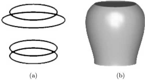
Fig. 1 Example of a PDE surface generated using the Bloor-Wilson PDE method. The boundary curves are shown in (a) and the corresponding PDE surface is shown in (b).
