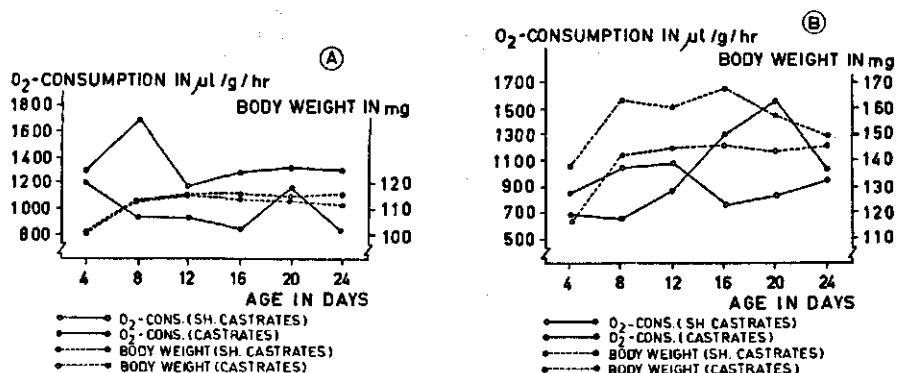
FIG. 6. Oxygen consumption and fresh body weight after castration in Leptinotarsa decemlineata . A, average curves derived from eight and nine male testictomates and sham testictomates respectively. B, average curves derived from seven and nine female ovariectomates and sham ovariectomates respectively.
