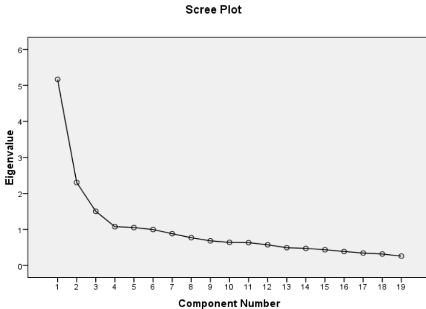
Figure 3. Scree plot of eigenvalue to component number
