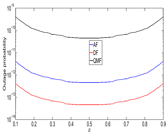
FIGURE 8. Outage probability as a function of \rho for (BFF,BF) scheme.
