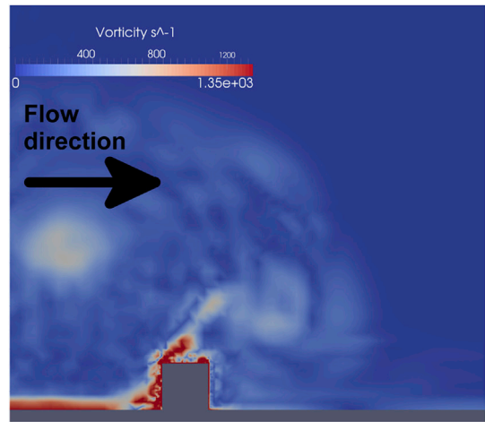
(a) Cube Building at 0^\circ - time t = 0.375s .
