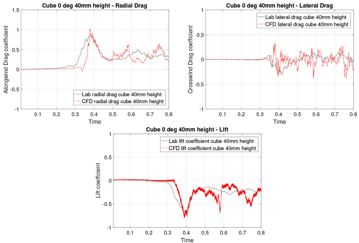
Fig. 10. Aerodynamic force coefficients for the cube building at 0° and at 40 mm height, compared to data from the laboratory simulations of Jesson et al. (2015).
