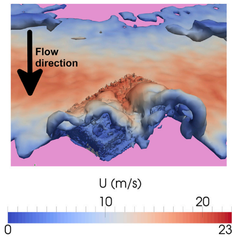
Fig. 23. The 550\text{s}^{-1} vorticity iso-surface coloured by velocity on the portal building at 45^\circ yaw angle: view from rear at point of maximum lift, t = 0.375\text{s} .
