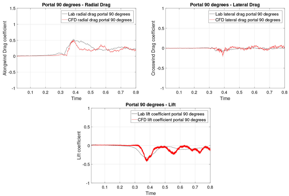
Fig. 14. Aerodynamic force coefficients for the portal building at 90° and at full height, compared to data from the laboratory simulations of Jesson et al. (2015).
