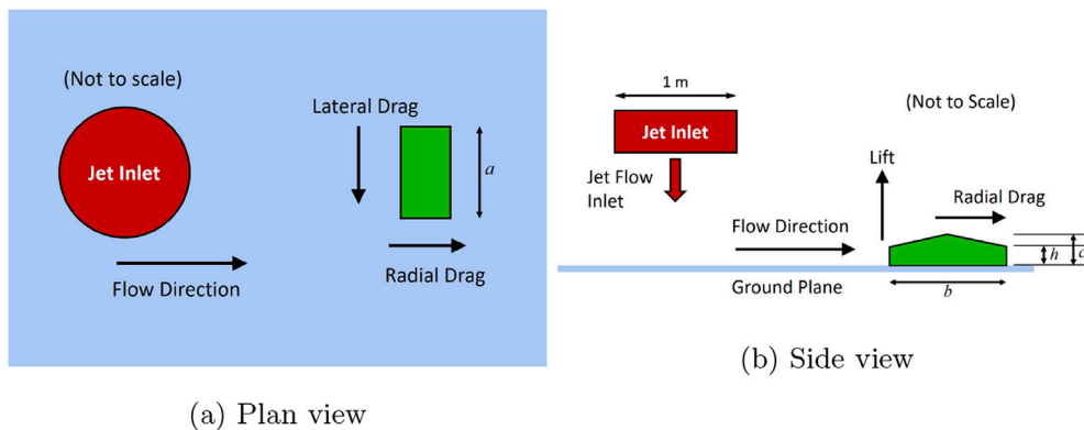
Fig. 5. The orientation of the radial, lateral and lift drag components in relation to the model buildings and experimental domain. Dimensions of portal building are a = 240\text{mm} , b = 130\text{mm} and c = 53\text{mm} , with eaves at height, h = 42\text{mm} . Cube building has dimensions, a = b = c = 60\text{mm} .
