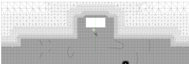
Fig. 2. The numerical model domain and mesh.
