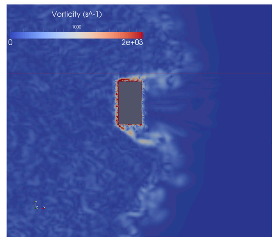
(b) Portal Building at 0^\circ - time t = 0.425\text{s} .
