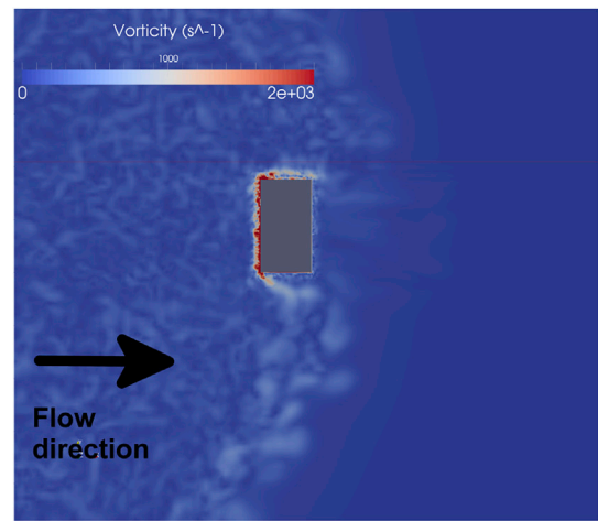
(a) Portal Building at 0^\circ - time t = 0.4\text{s} .
