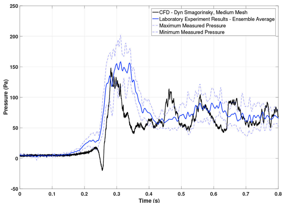
Fig. 6. Comparison of Measured and Predicted Pressure in centre of Centre Face of Cube, 0^\circ full height configuration.
