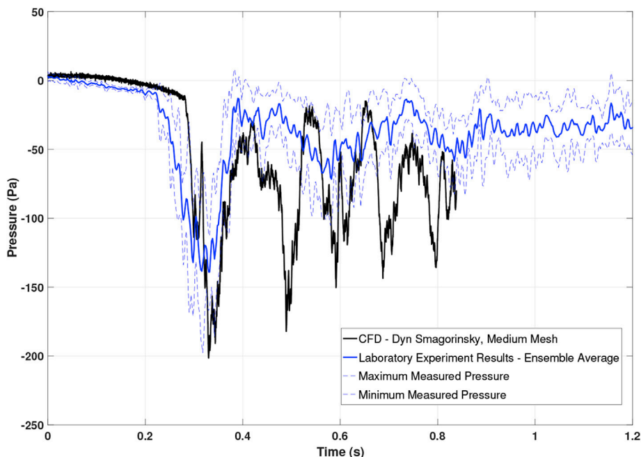
Fig. 7. Comparison of Measured and Predicted Pressure in centre of Roof Face of Cube, 0° full height configuration.
