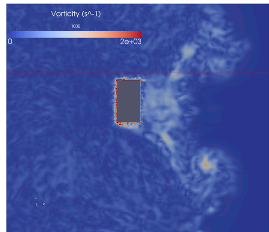
(c) Portal Building at 0^\circ - time t = 0.475\text{s} .
