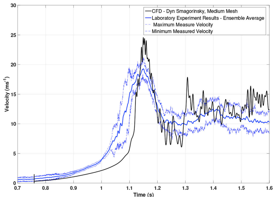
Fig. 8. Comparison of Measured and Predicted Velocity at X/D = 1.5 on jet centreline at a height of Z/D = 0.03 from ground plane.
