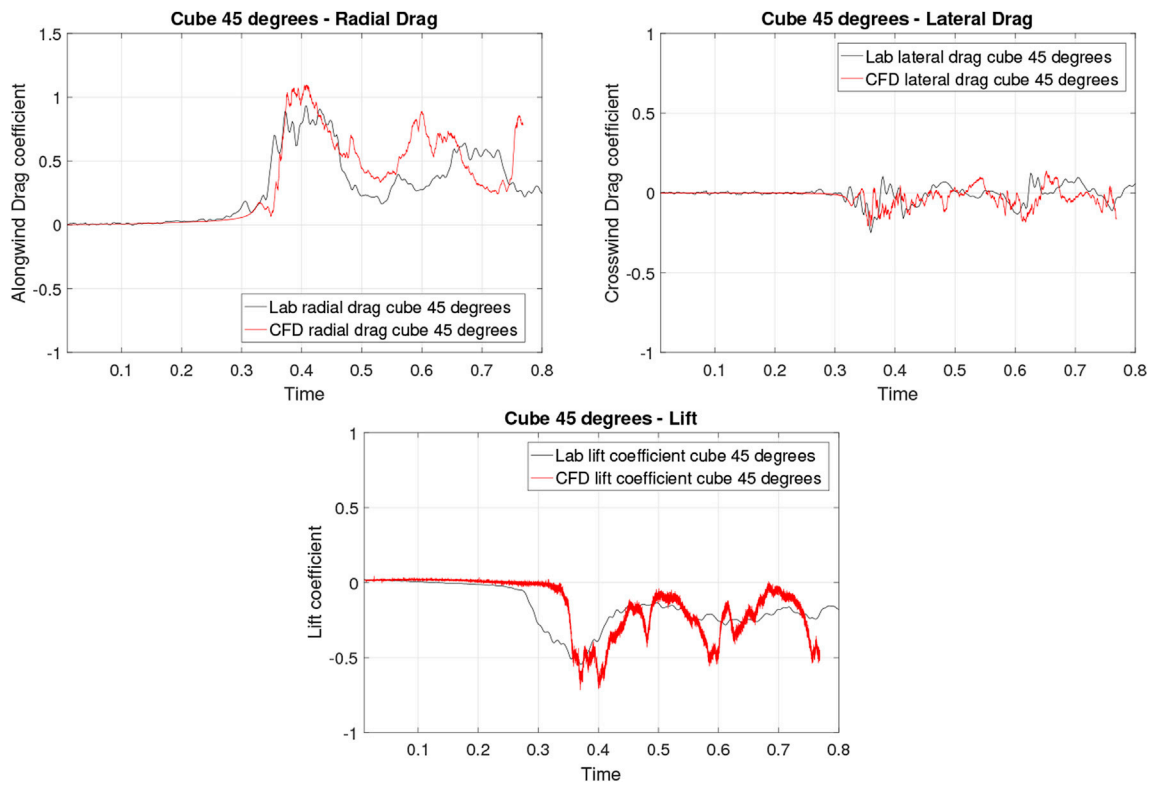
Fig. 11. Aerodynamic force coefficients for the cube building at 45° and at full height, compared to data from the laboratory simulations of Jesson et al. (2015).
