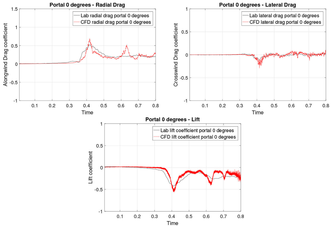
Fig. 12. Aerodynamic force coefficients for the portal building at 0° and at full height, compared to data from the laboratory simulations of Jesson et al. (2015).
