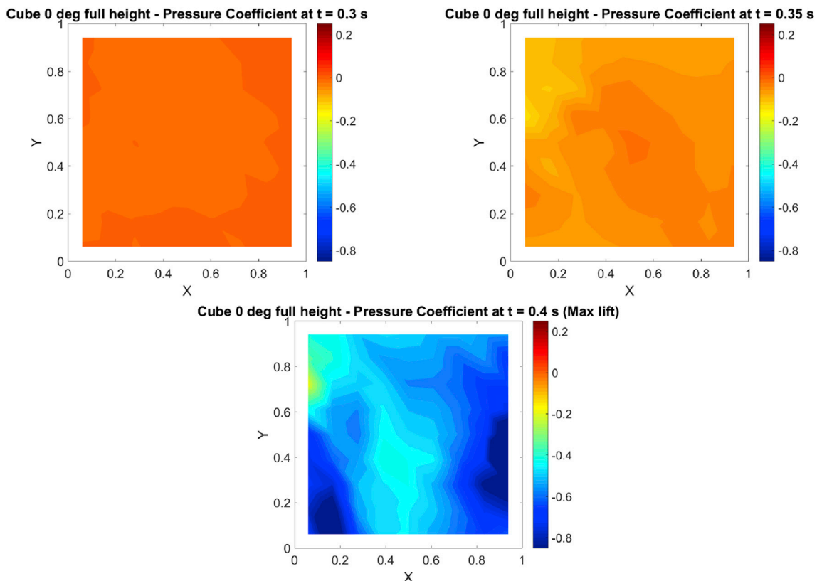
Fig. 16. Pressure on roof of cube at 0° yaw angle: results of CFD analysis.
