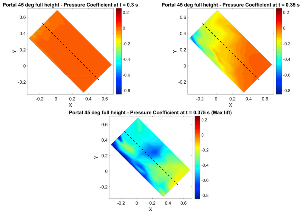
Fig. 19. Pressure on roof of portal building at 45° yaw angle: results of CFD analysis.
