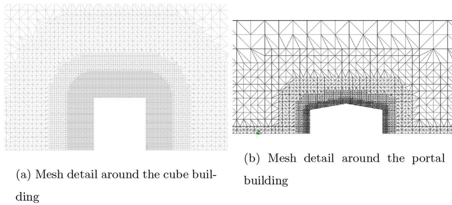
Fig. 3. Numerical model domain and mesh with detail around a) the cube and b) the portal building.
