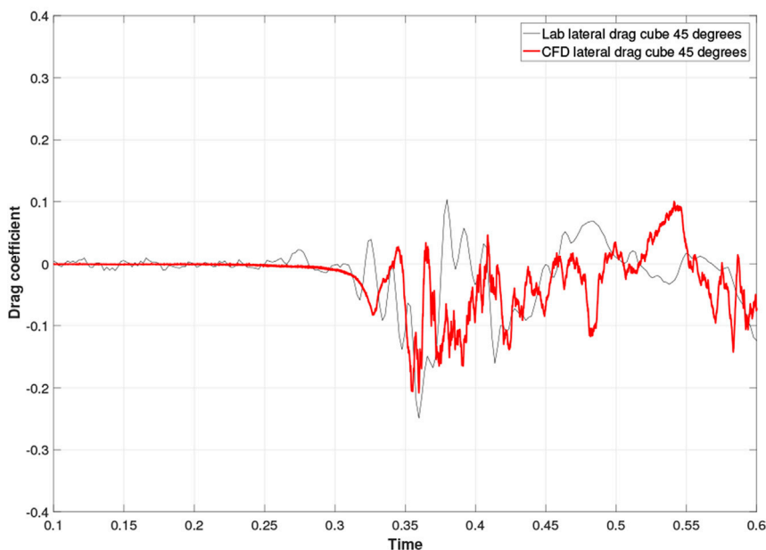
(b) Cube at 45° Lateral Drag Coefficient.
