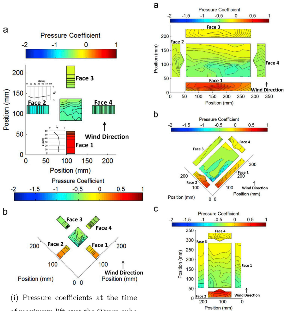
(ii) Pressure coefficients at the time of maximum lift over the portal building at 0° (a), 45° (b) and 90° (c) yaw angles (Reproduced from Jesson et al. (2015)).
