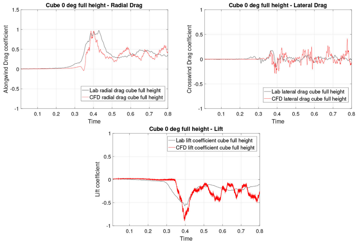
Fig. 9. Aerodynamic force coefficients for the cube building at 0° and at full height, compared to data from the laboratory simulations of Jesson et al. (2015).
