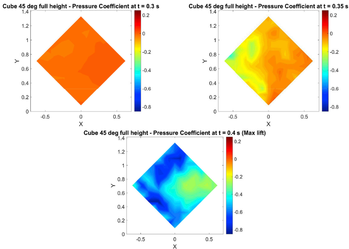
Fig. 17. Pressure on roof of cube at 45° yaw angle: results of CFD analysis.
