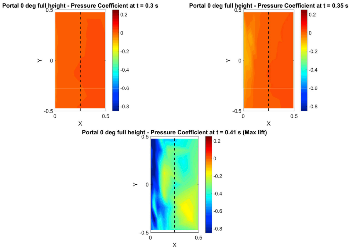
Fig. 18. Pressure on roof of portal building at 0° yaw angle: results of CFD analysis.
