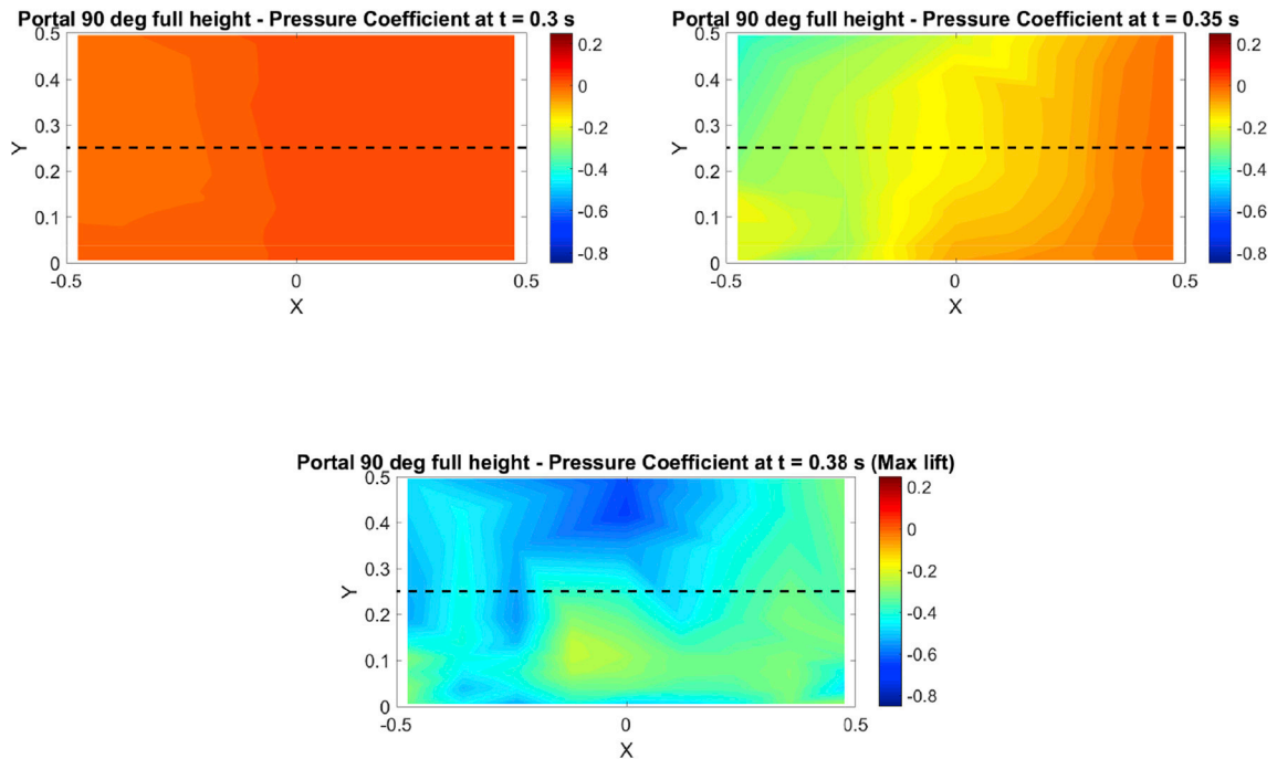
Fig. 20. Pressure on roof of portal building at 90° yaw angle: results of CFD analysis.
