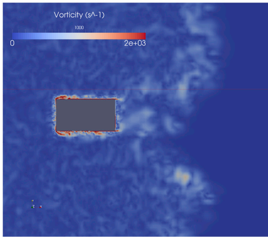
(b) Portal Building at 90^\circ - time t = 0.45s .
