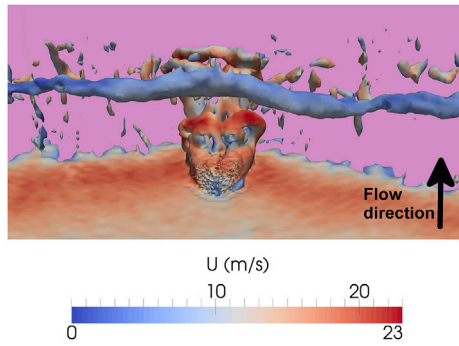
Fig. 24. The 550\text{s}^{-1} vorticity iso-surface around the cube building at the 45^\circ yaw angle - view from front at time t = 0.4\text{s} .
