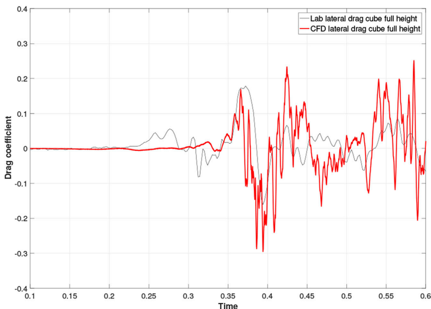
(a) Cube at 0° Lateral Drag Coefficient.
