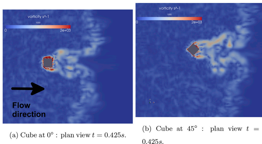
Fig. 21. The vorticity contours at a height of 30mm illustrating the vortex shedding on the sides of the cube building at the 0° and 45° yaw angles.
