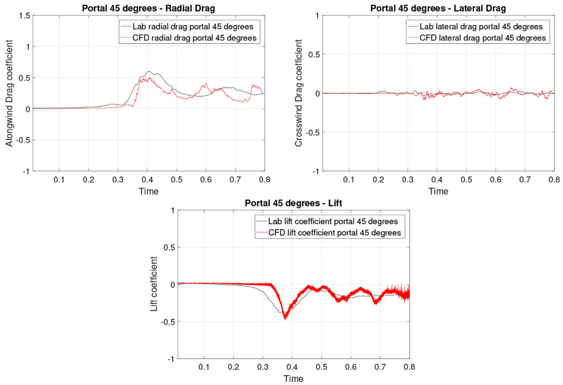
Fig. 13. Aerodynamic force coefficients for the portal building at 45° and at full height, compared to data from the laboratory simulations of Jesson et al. (2015).
