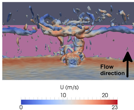
Fig. 25. The 550\text{s}^{-1} vorticity iso-surface around the cube building at the 0^\circ yaw angle - view from front at t = 0.425\text{s} .
