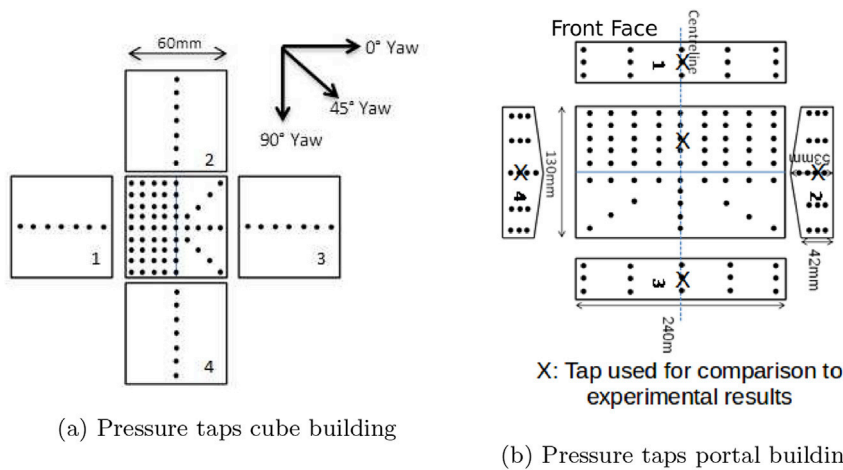
Fig. 4. The location of the pressure taps on the study of Jesson et al. (2015) for a) the cube and b) the portal building.
