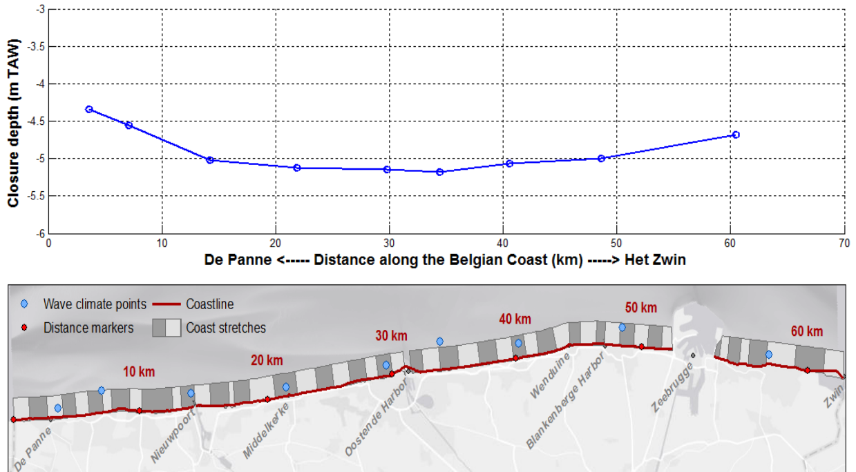
Figure 8 – Closure depth (in m TAW) along the Belgian coast, as calculated with Hallermeier 1981.
