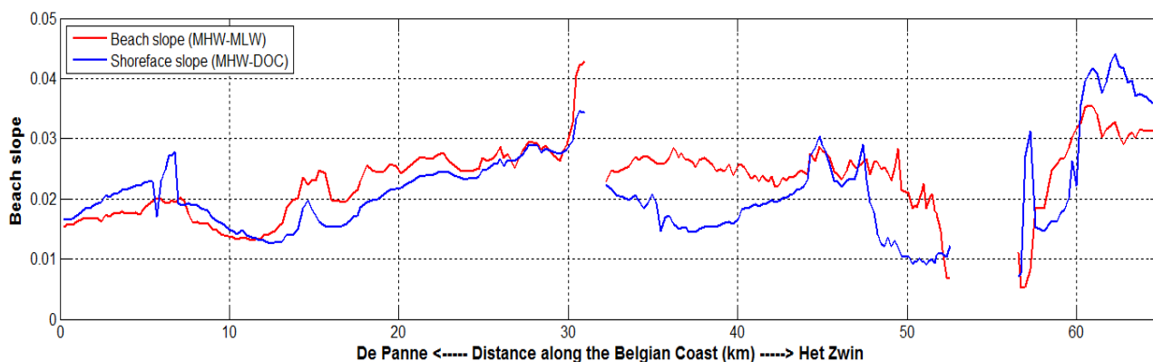
Figure 11 – Beach slopes along the Belgian Coast.
