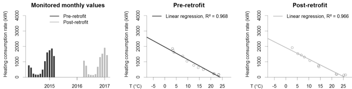
Fig. 7. Hospital Building data from measurement, with monthly resolution.
