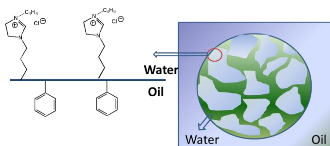
Scheme 1. Schematic structure of IL-Janus nanosheets and formation of Pickering emulsions.
