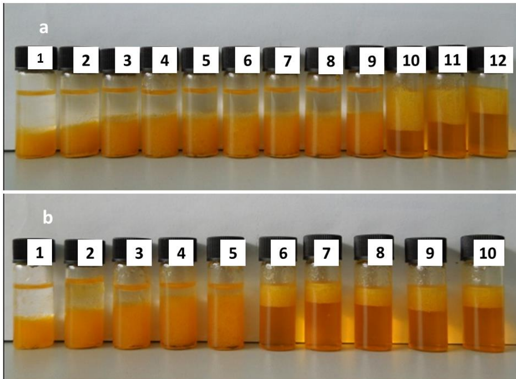
Fig. 5. Photographs of water-toluene emulsions (2.0 mL) stabilized by 2.0 mg CI-based IL-Janus nanosheets with various volume fraction of water ( \Phi_w ) after standing for 30 d.: a. water as initial location, No. 1-12: \Phi_w = 0.300, 0.400, 0.425, 0.450, 0.475, 0.480, 0.485, 0.490, 0.495, 0.500, 0.600 and 0.700 , No.1-9: W/O type emulsions, No. 10-12: O/W type emulsions; b. toluene as initial location, No. 1-10: \Phi_w = 0.300, 0.400, 0.500, 0.600, 0.700, 0.705, 0.710, 0.715, 0.720 and 0.725 , No.1-5: W/O type emulsions, No. 6-10: O/W type emulsions.
