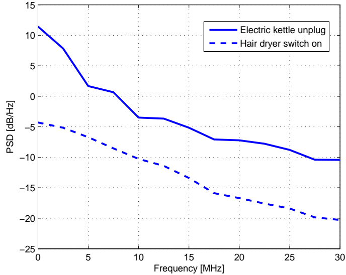
Figure 3.6: PSD of the impulsive noises from the power line (Fig. 3.5).
