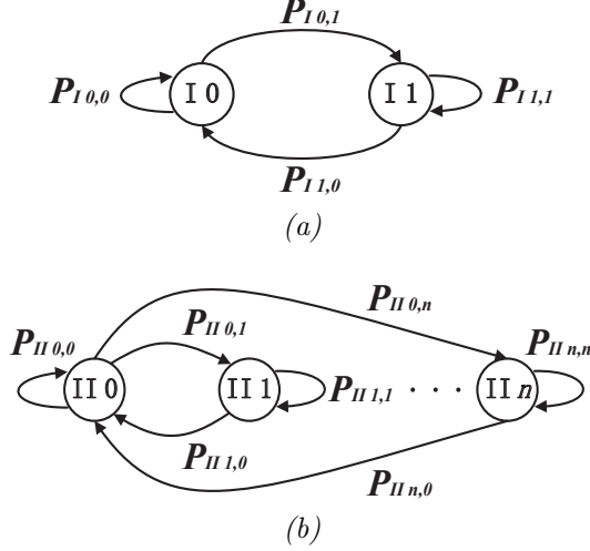
Figure 3.9: (a) First level Markov chain for modelling the occurrence of bursts (‘ I 0 ’—non-burst state; ‘ I 1 ’—burst state) (b) Second level Markov chain for modelling the occurrence of individual impulses in a burst (‘ II 0 ’—non-impulse state; ‘ II l ’—impulse states with different impulse variances ( l = 1, \dots, n )).
