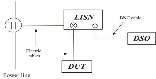
Figure 3.2: Measurement setup for PLC noise at source.
